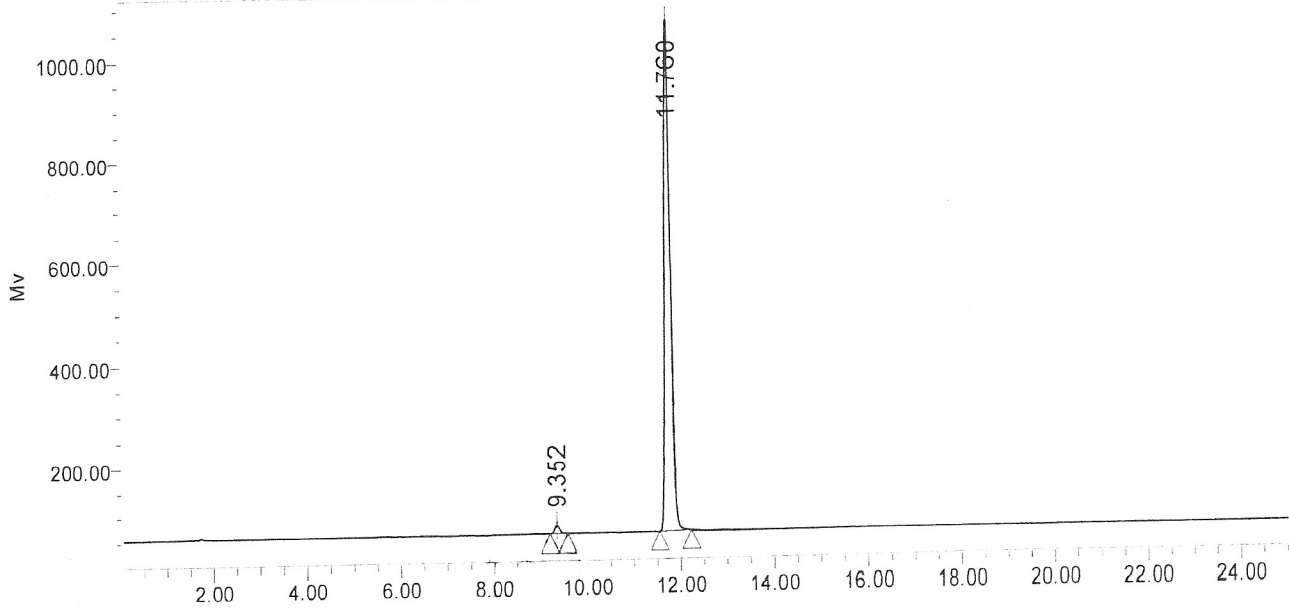
Auto-Scaled Chromatogram
